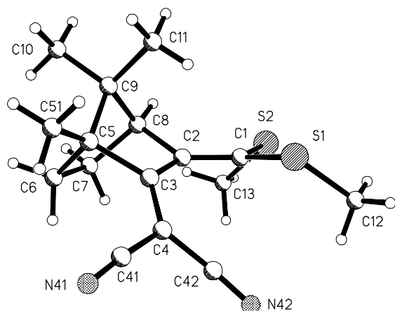
Fig. 1 Molecular structure of compound (1 R ,4 S )- 2 (arbitrary numbering). Selected bond lengths (Å), angles ( ^\circ ) and dihedral angles ( ^\circ ): C(1)–C(2) 1.353(4), C(2)–C(3) 1.466(3), C(3)–C(4) 1.358(3), C(4)–C(41) 1.432(4), C(4)–C(42) 1.433(4), C(1)–S(2) 1.755(2), C(1)–S(1) 1.755(3), S(1)–C(1)–C(2) 119.8(2), C(1)–C(2)–C(3) 128.5(2), C(2)–C(3)–C(4) 126.6(2), C(3)–C(4)–C(42) 122.3(2), S(2)–C(1)–C(2)–C(8) -25.9(4) , S(1)–C(1)–C(2)–C(3) -22.5(3) , C(1)–C(2)–C(3)–C(4) -40.2(4) , C(2)–C(3)–C(4)–C(42) -172.6(2) , C(5)–C(3)–C(4)–C(41) -9.1(4) .
