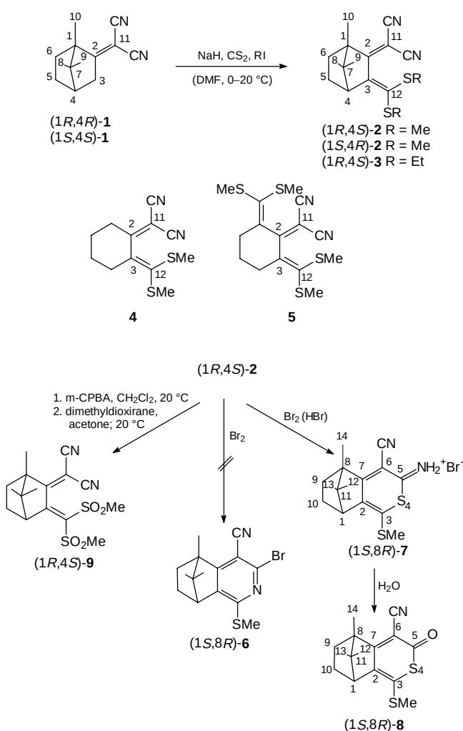
Scheme 1 Synthesis and reactions of bornane with integrated push–pull butadienes
